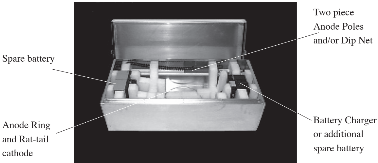
Carrying case without the 12-B Electrofisher. Shows placement of the spare battery, anode ring and pole, rat-tail cathode, and battery charger.
