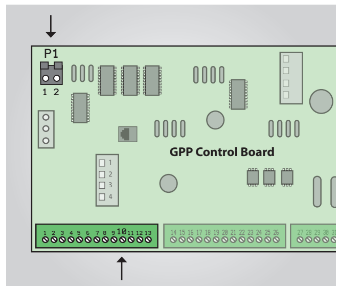
Location of 2 pin connector on upper left hand corner of board and location of terminal 10 on terminal strip.
