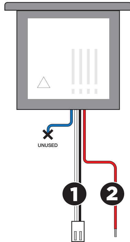
Diagram showing wiring configuration as supplied by Smith-Root.
